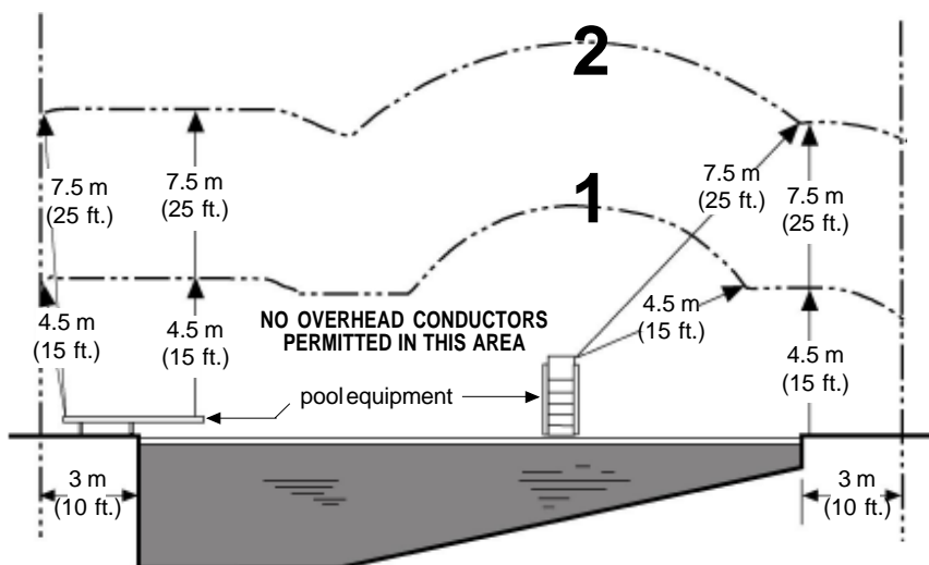
FIGURE 3 - Overhead Conductors
